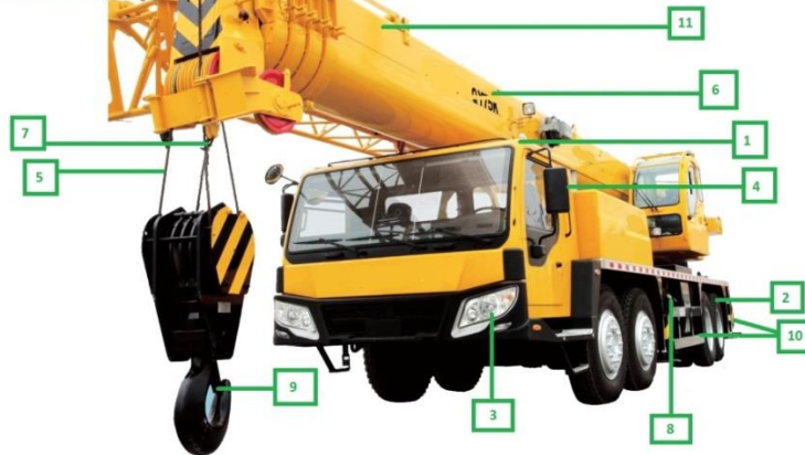
Mobile Crane Inspection Diagram
